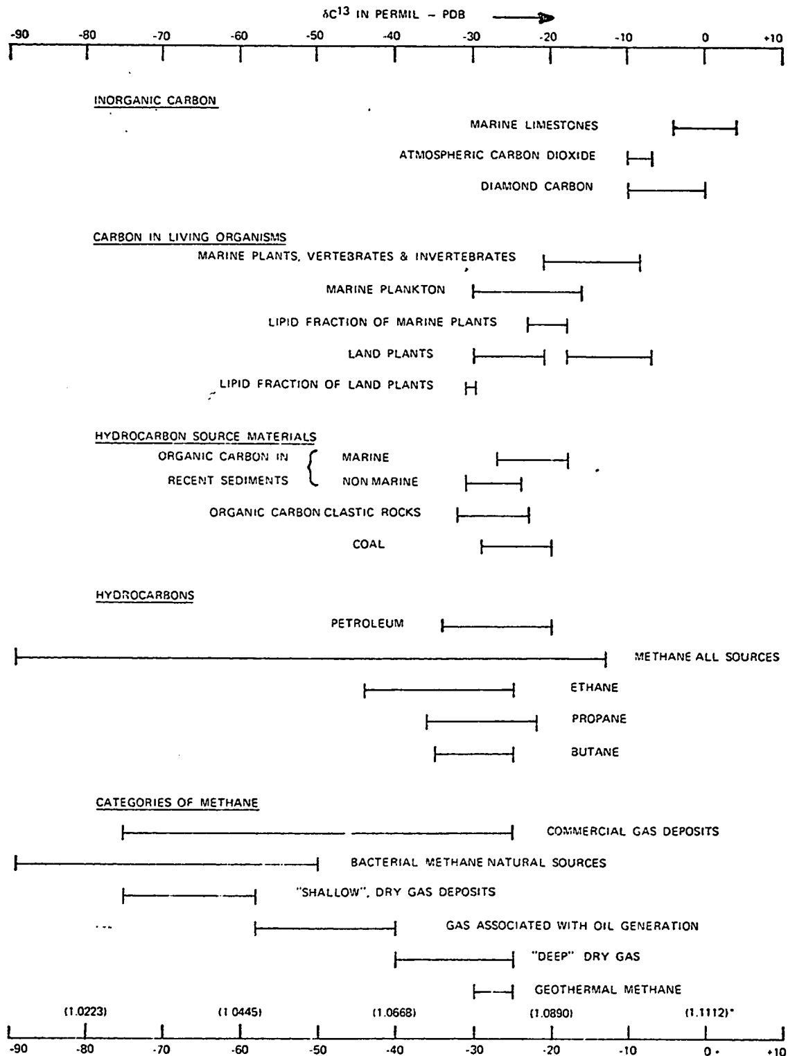
Fig. 1. Carbon isotope ranges of carbonaceous materials (after Fuex, 1977).
