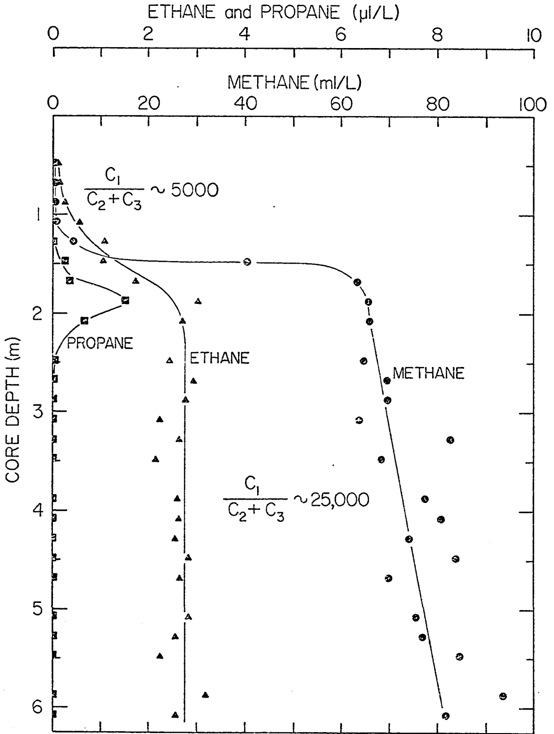
Fig. 20. Interstitial methane, ethane, and propane at Station 58.
