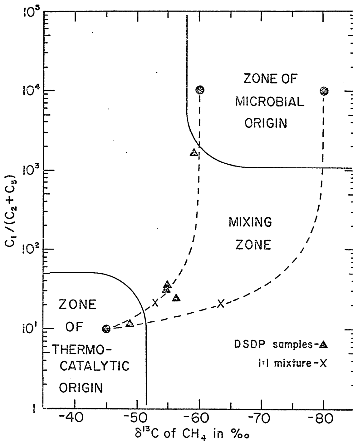
Fig. 4. Model for source characterization of marine hydrocarbon gases.
