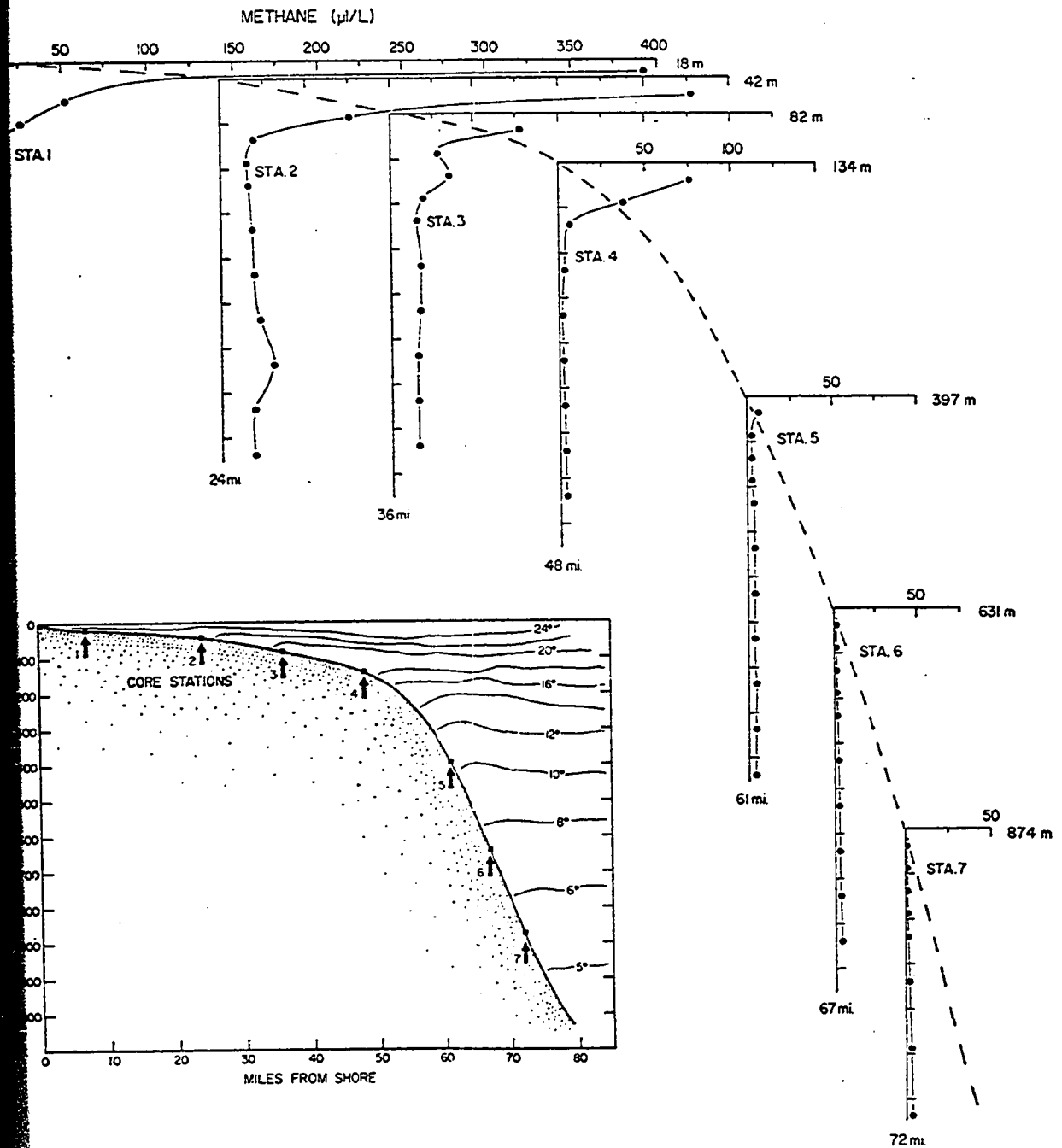
Interstitial methane along Transect I, positioned on the sea floor contour. Inset shows the general temperature structure of the area in spring.
