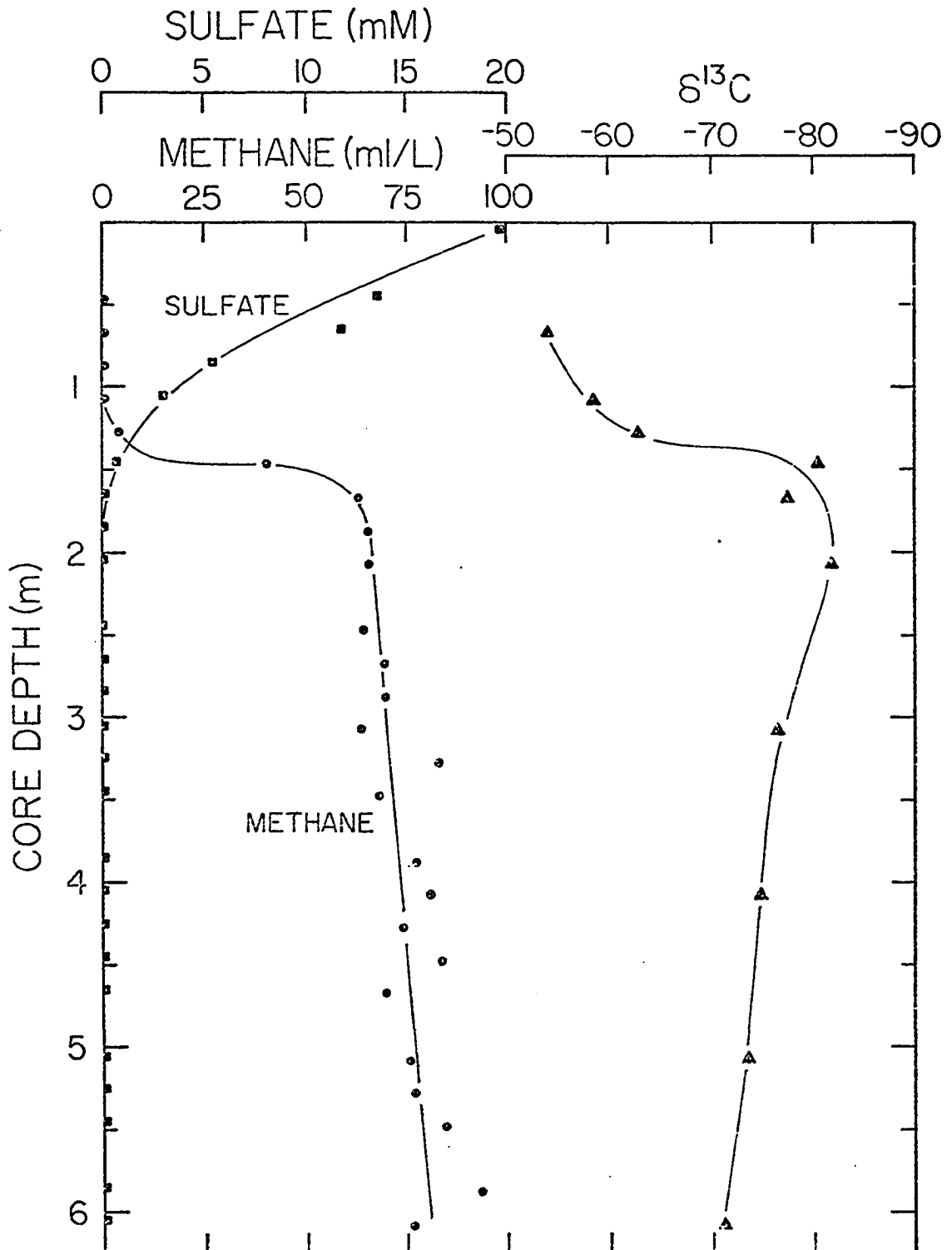
Fig. 19. Interstitial methane and sulfate at Station 58.
