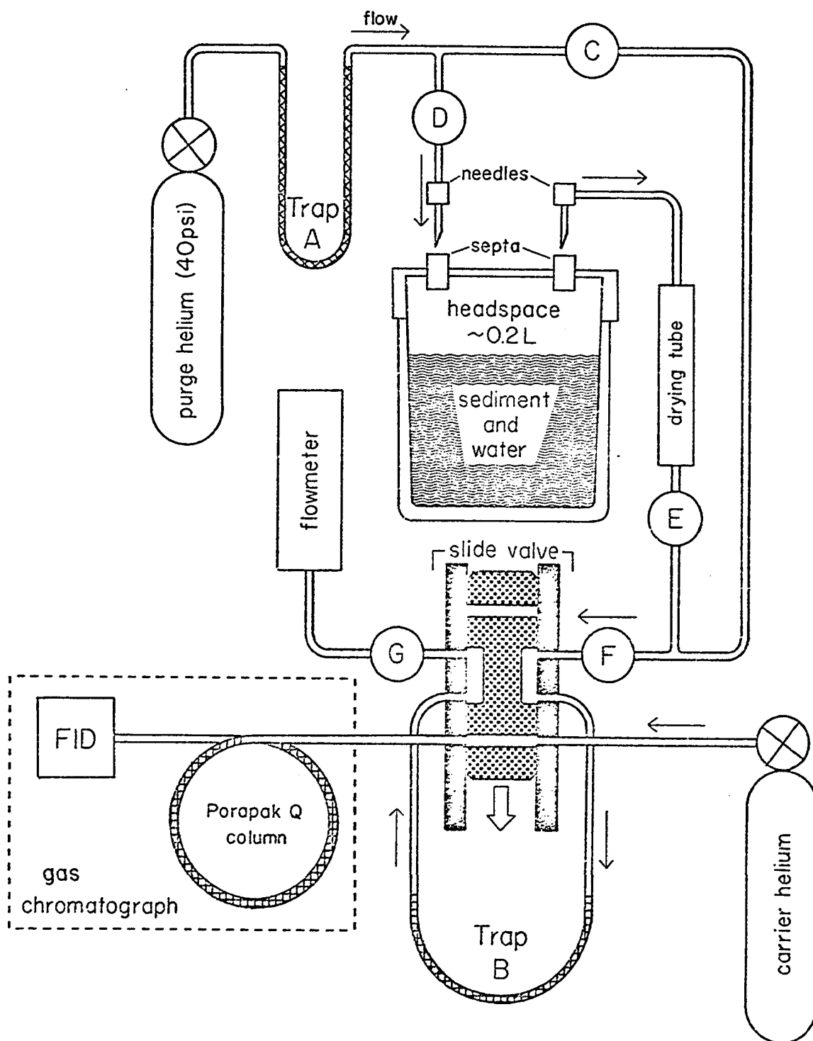
Fig. 9. Schematic of the system used for analysis of sediment light hydrocarbons.
