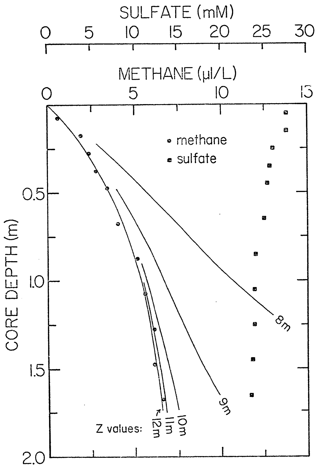
Fig. 18. Interstitial methane and sulfate at Station 57.
