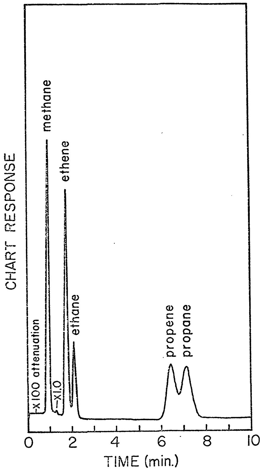
Fig. 10. Chromatogram of sediment light hydrocarbons.
