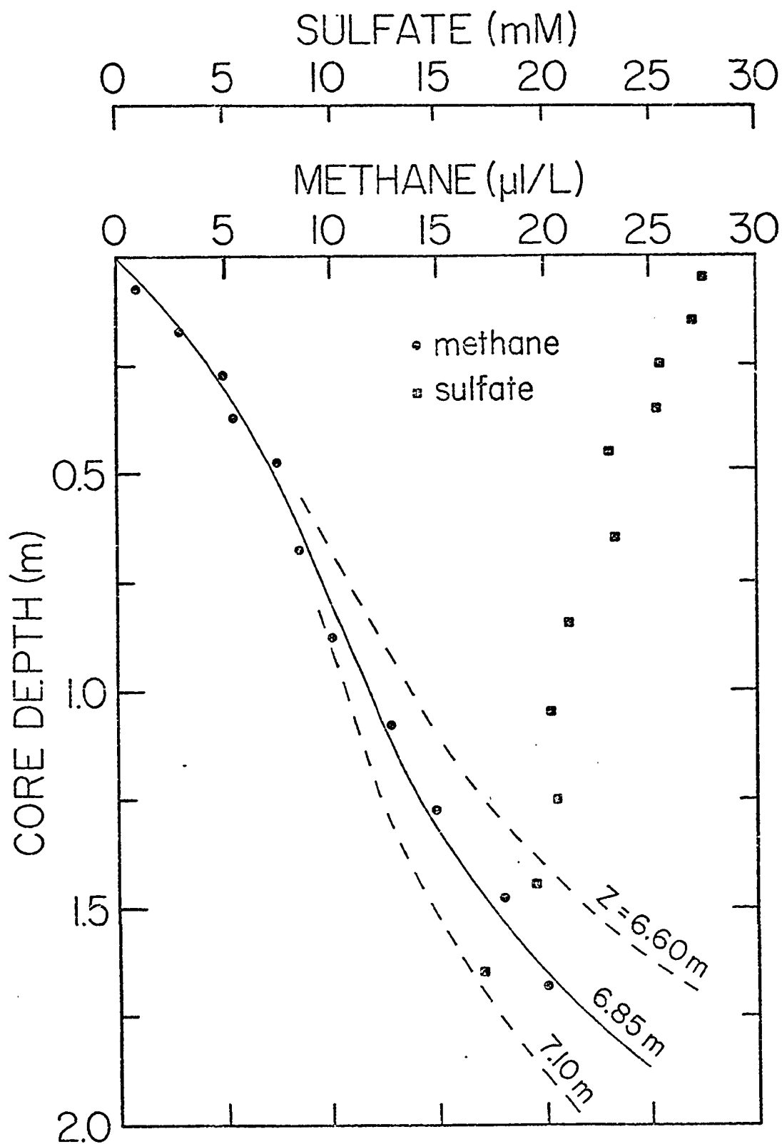
Fig. 17. Interstitial methane and sulfate at Station 56.
