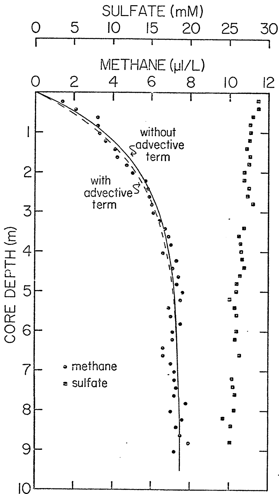
Fig. 15. Interstitial methane and sulfate at Station 54.
