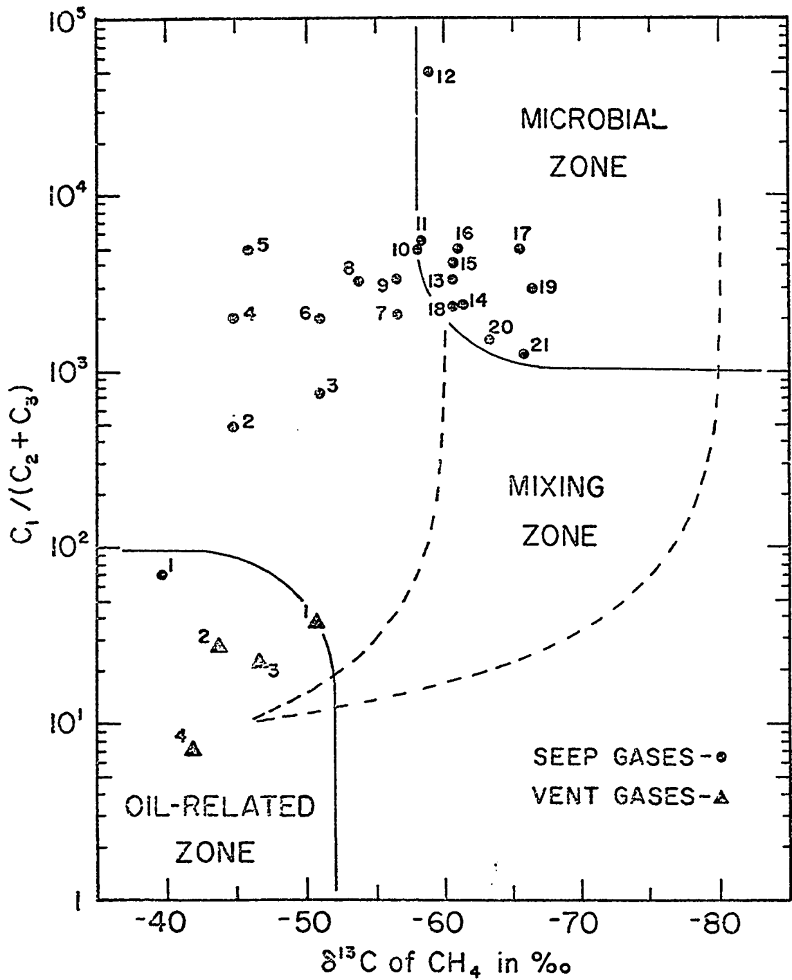
Fig. 6. C_1/(C_2+C_3) vs. \delta^{13}C for seep gas samples listed in Table 1.
