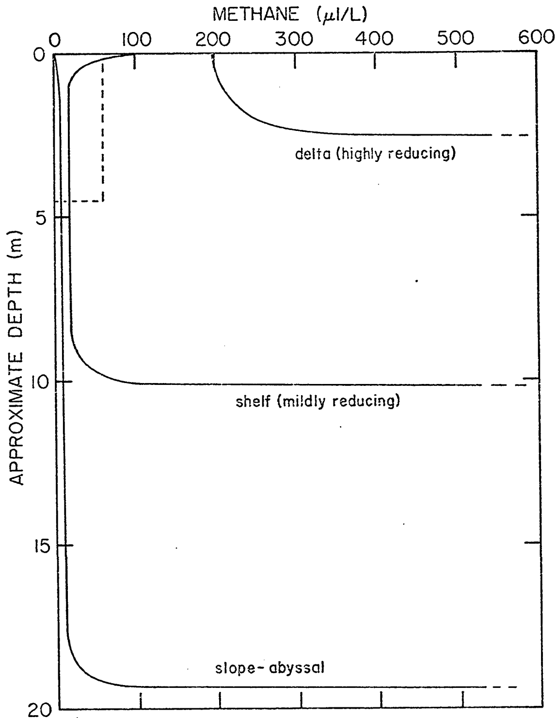
Fig. 24. Idealized methane profiles in the upper 20 meters of various sedimentary environments (inset corresponds to Fig. 23).
