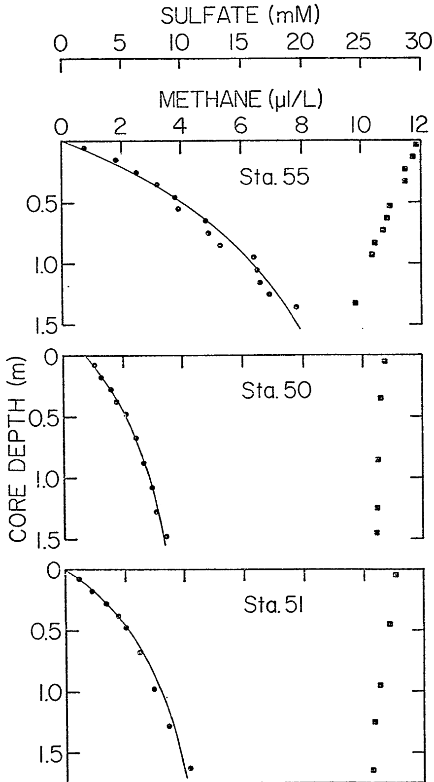
Fig. 16. Interstitial methane and sulfate at Stations 50, 51 and 55.
