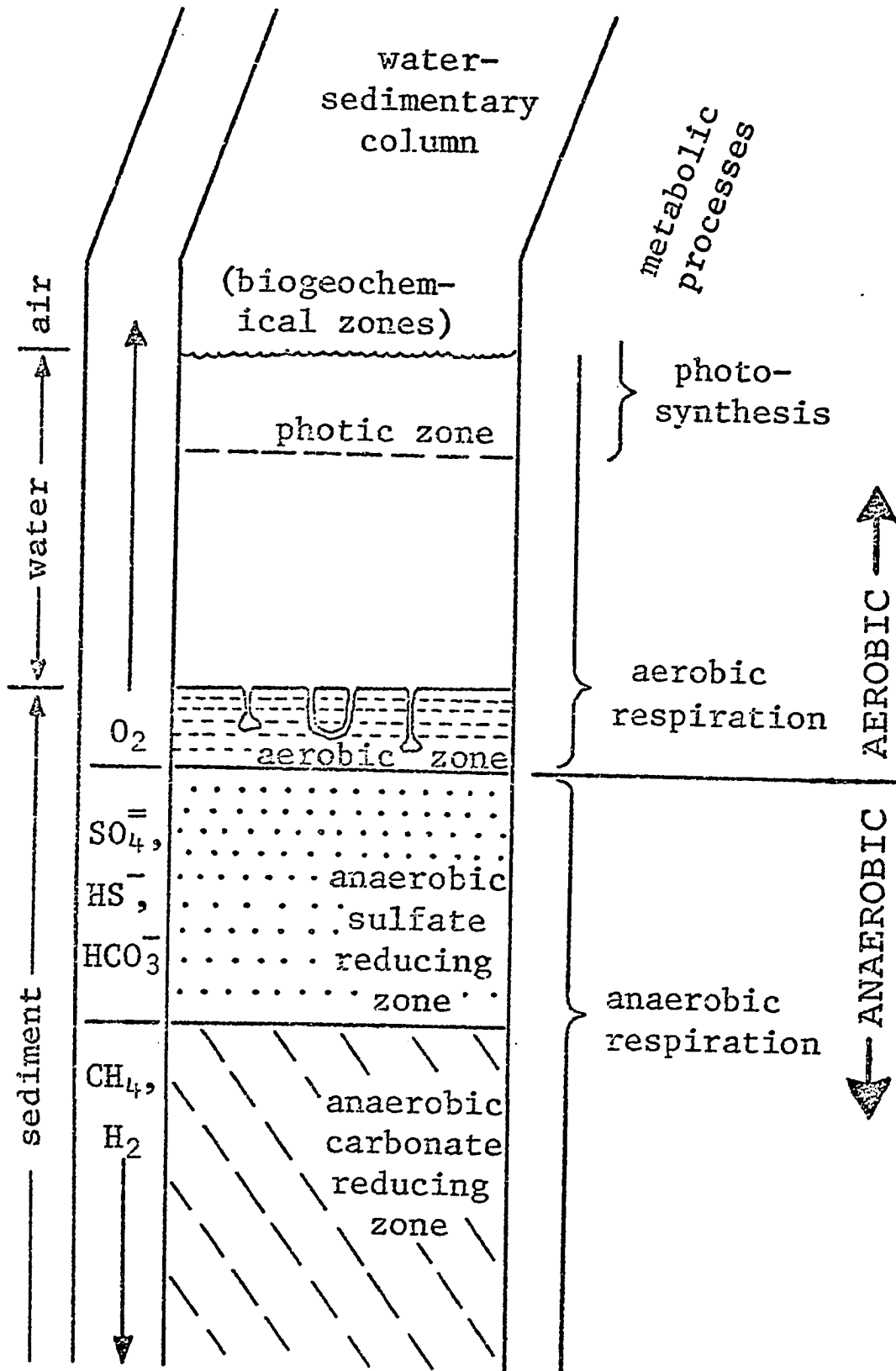
Fig. 8. An idealized cross section of an open marine organic-rich (reducing) sedimentary environment (after Claypool and Kaplan, 1974).
