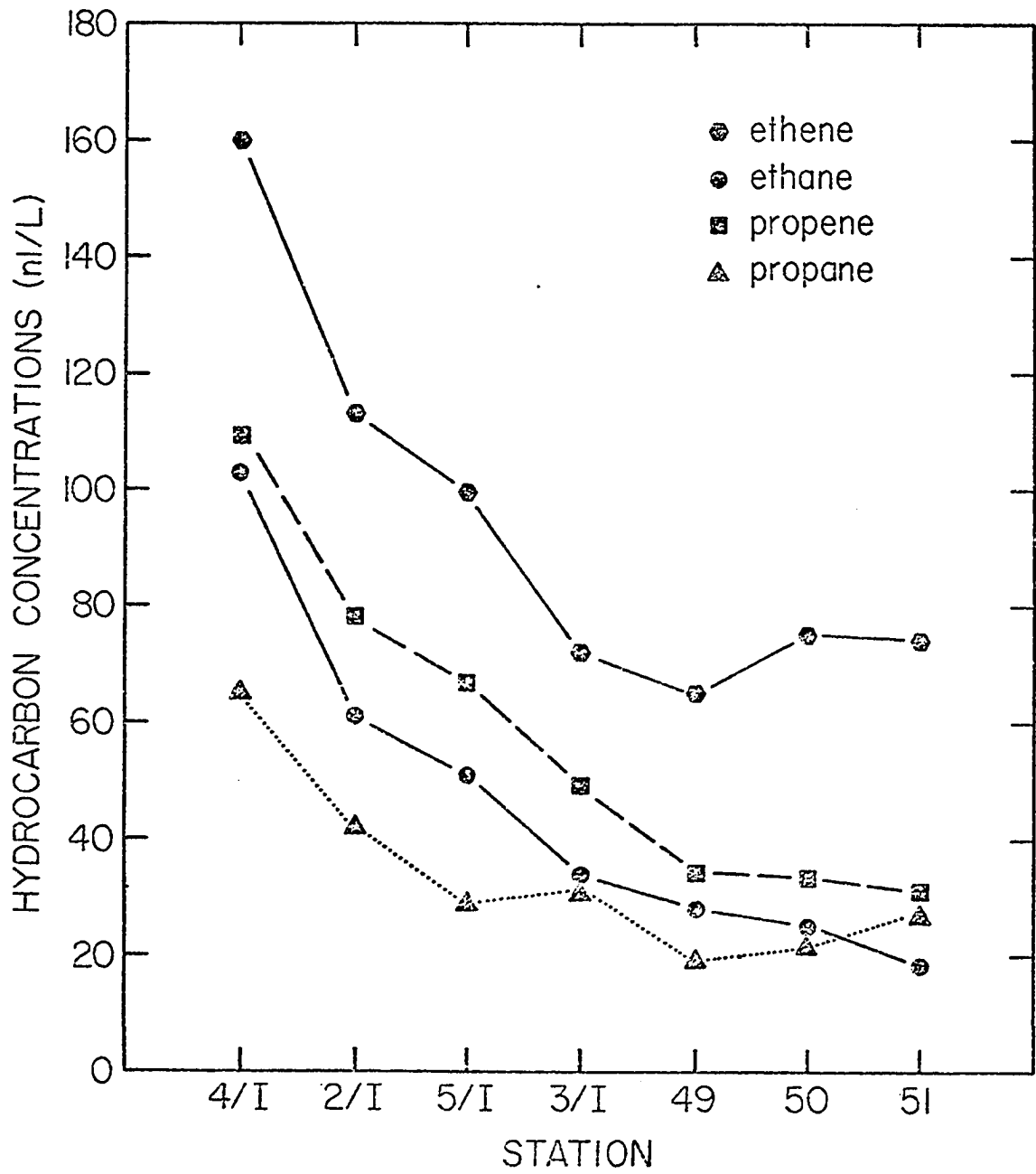
Fig. 22. Average concentrations of the C 2 and C 3 hydrocarbons at Transect I stations.
