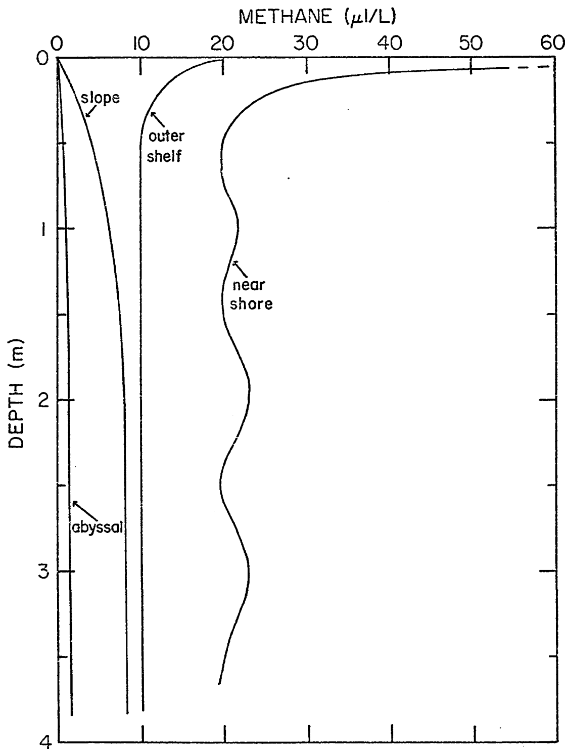
Fig. 23. Schematic diagram of methane variations in the upper 4 meters of sediment.
